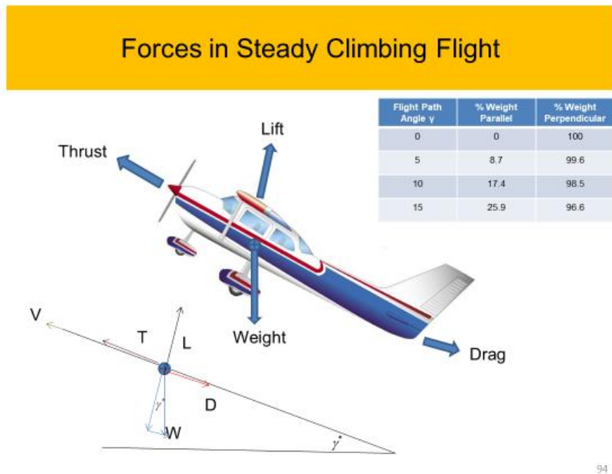
Figure 14: Forces in a Steady Climb
