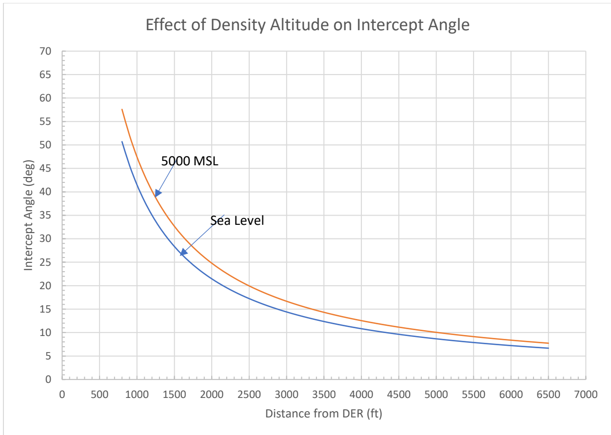
Figure 12: Effect of Density on Intercept Angle
