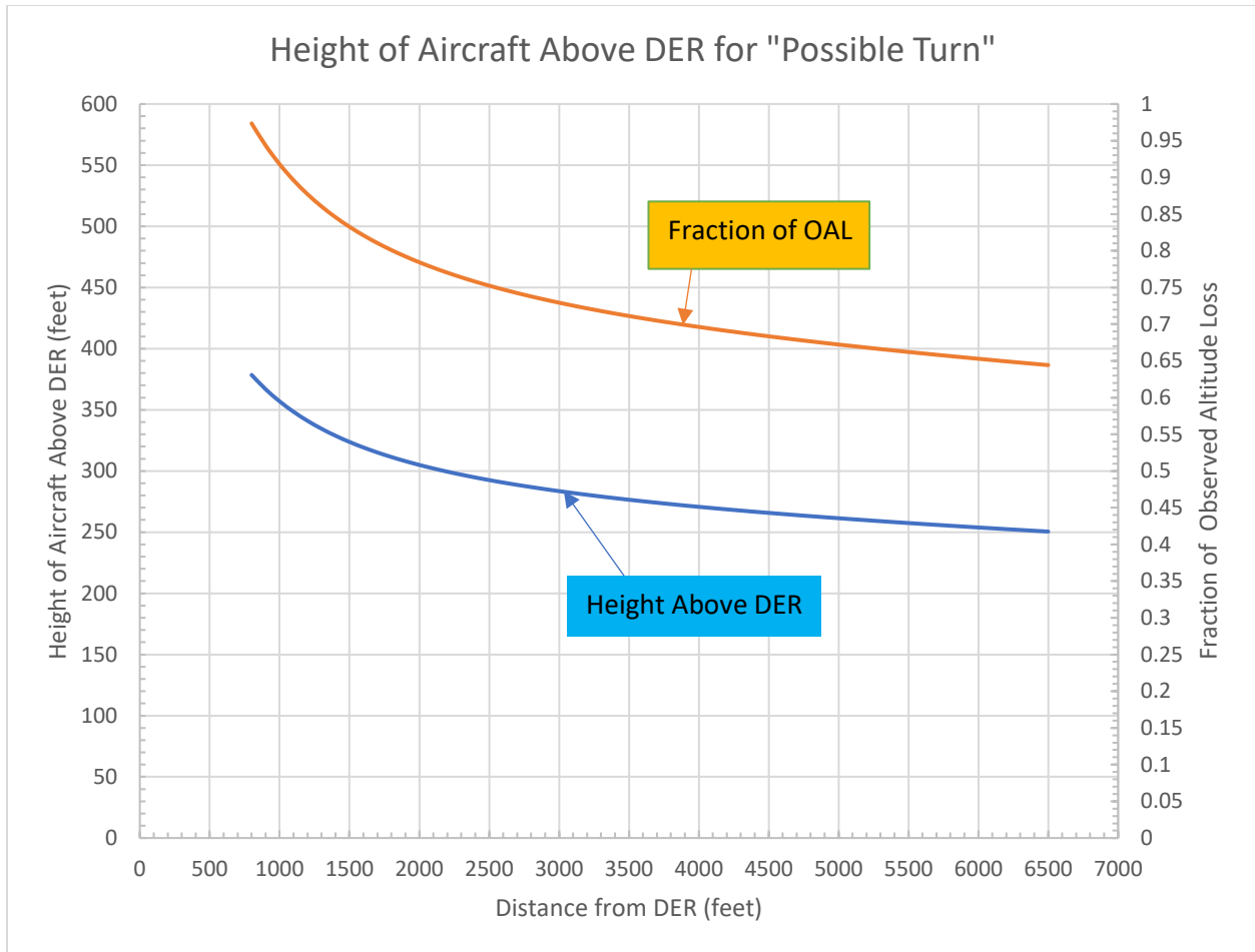
Figure 18: C-172 Required Height over DER for a PSTM
