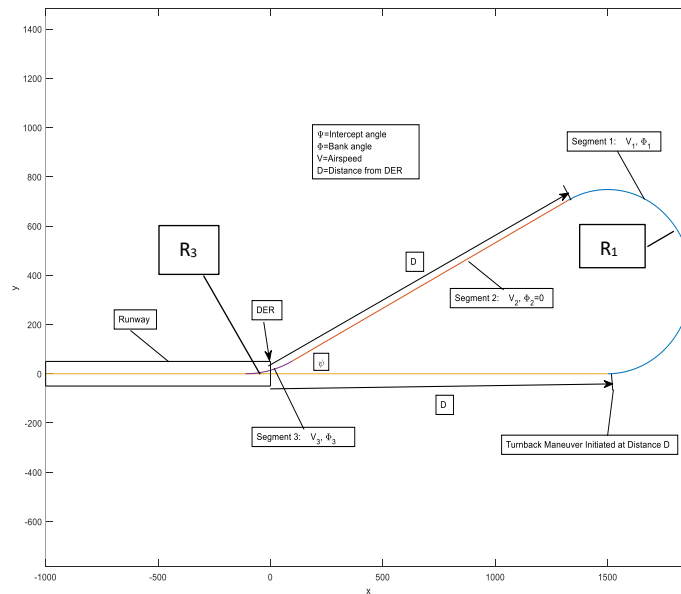
Figure 1: Geometry of the Teardrop Turnback Maneuver.
